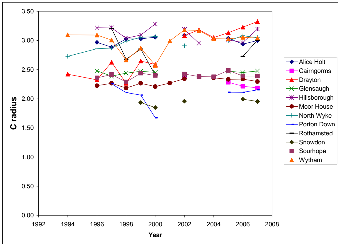
Fig. 3.3 Mean C radius of species in plot by year for each site.
