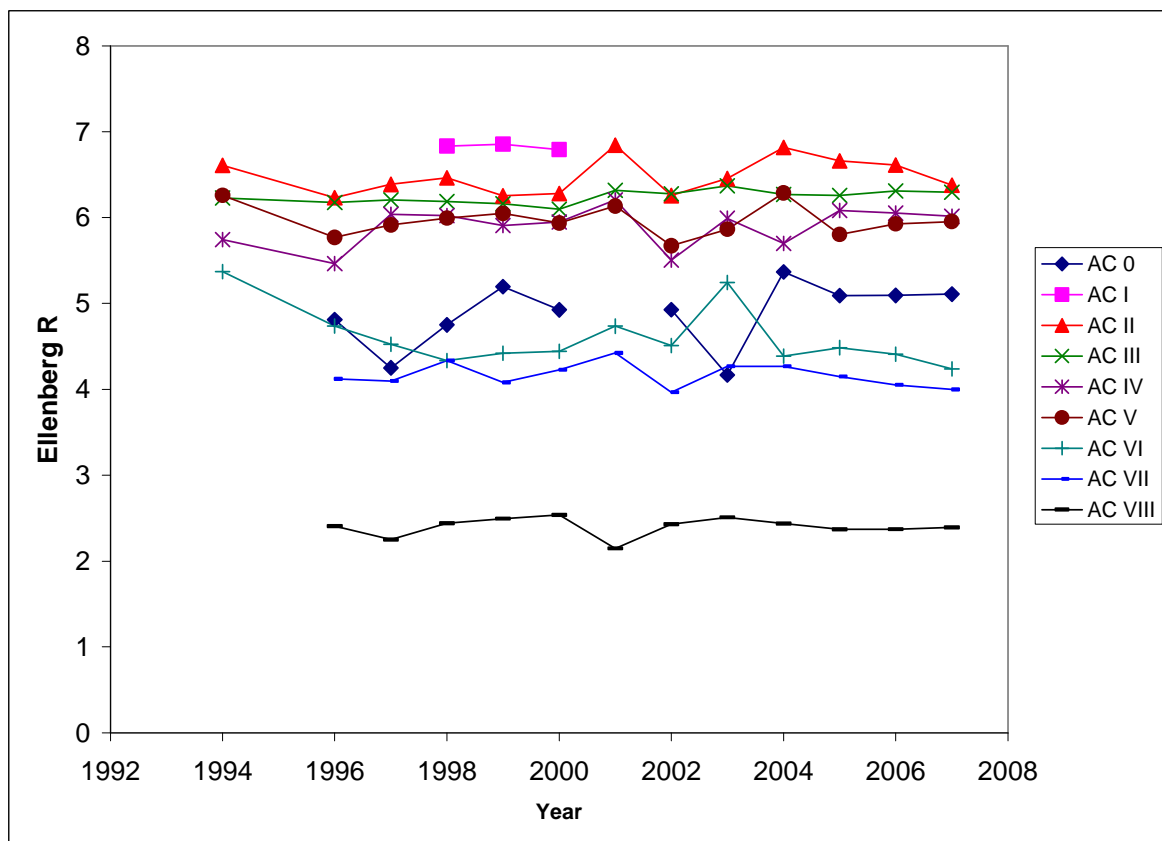
Fig. 3.10 Mean Ellenberg R of species in plot by year for aggregate vegetation classes
