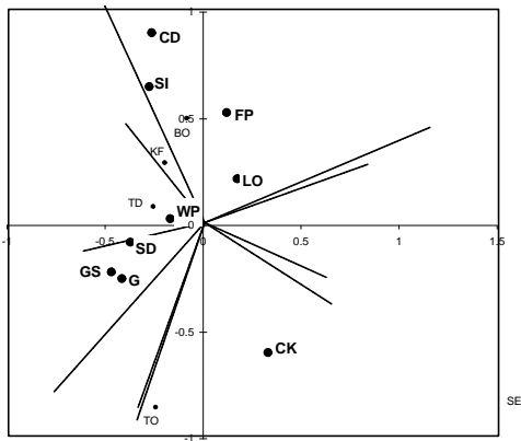
8. Ordination plot for near-passerines
