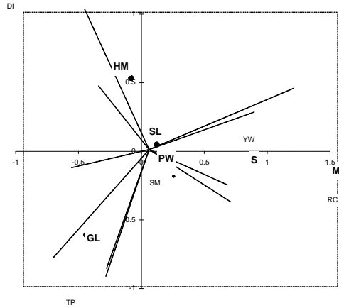
9. Ordination plot for larks, hirundines, pipits, wagtails and Dipper
