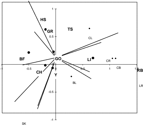
14. Ordination plot for sparrows, finches and buntings
