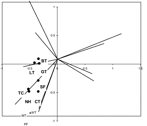
12. Ordination plot for flycatchers, tits, Nuthatch & Treecreeper
