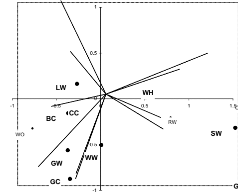
11. Ordination plot for warblers and Goldcrest
