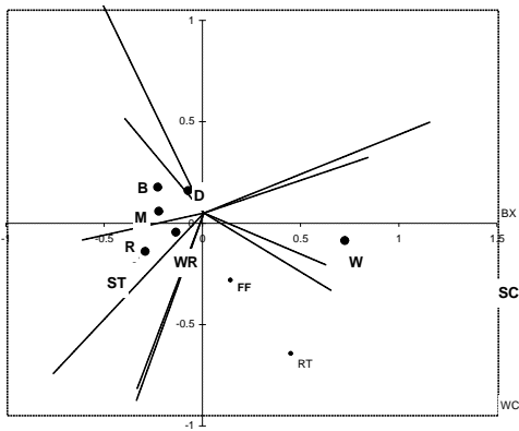
10. Ordination plot for Wren, Dunnock, chats and thrushes
