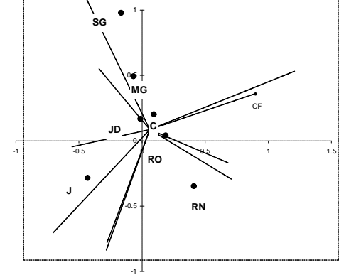
13. Ordination plot for crows and Starling
