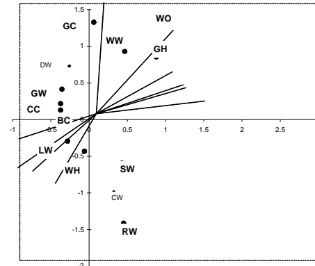
13. Ordination plot for crows and Starling
