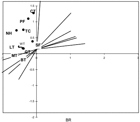
14. Ordination plot for sparrows, finches and buntings
