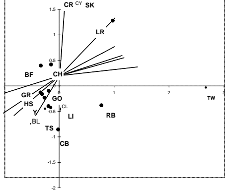
14. Ordination plot for sparrows, finches and buntings
