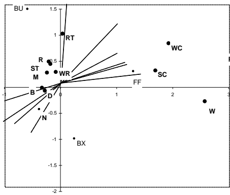
12. Ordination plot for flycatchers, tits, Nuthatch & Treecreeper
