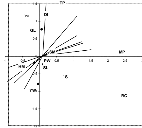
11. Ordination plot for warblers and Goldcrest
