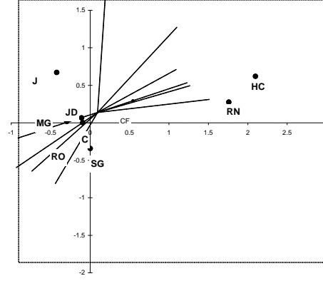
13. Ordination plot for crows and Starling
