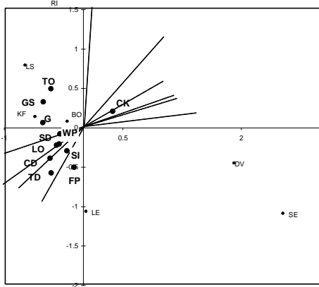
10. Ordination plot for Wren, Dunnock, chats and thrushes
