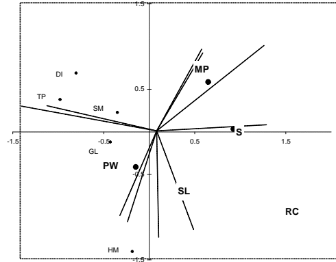
11. Ordination plot for warblers and Goldcrest
