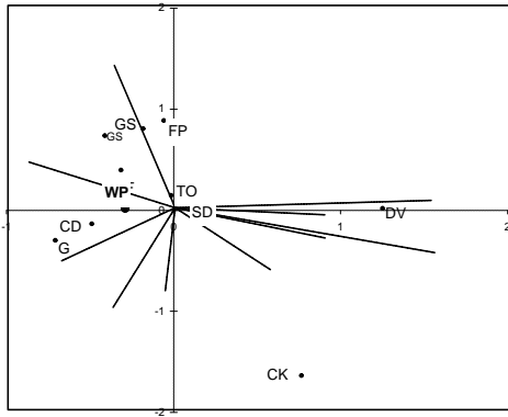
8. Ordination plot for near-passerines
