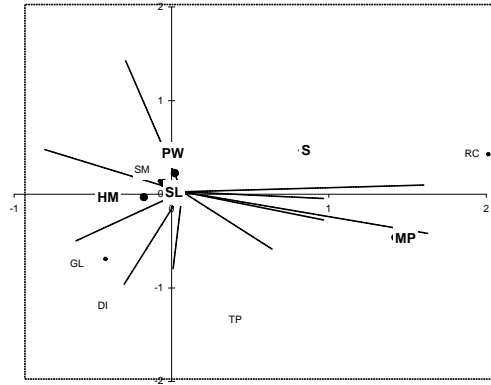
9. Ordination plot for larks, hirundines, pipits, wagtails and Dipper
