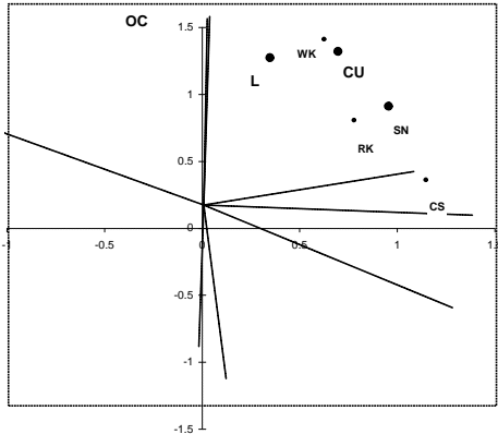
6. Ordination plot for waders
