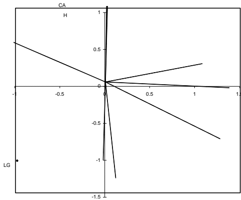
4. Ordination plot for raptors
