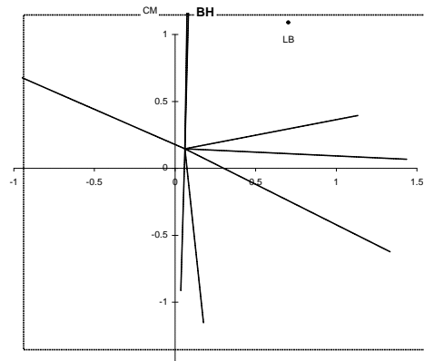
7. Ordination plot for skuas, gulls, terns and auks
