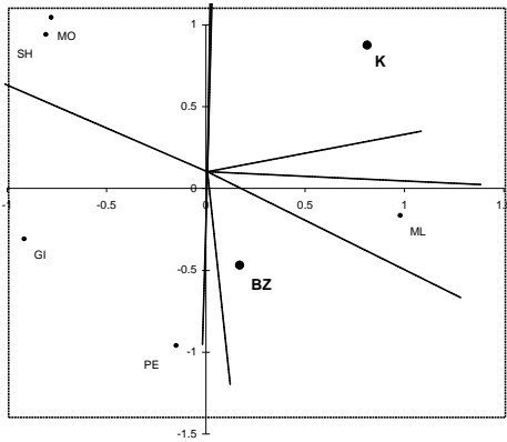
4. Ordination plot for raptors
