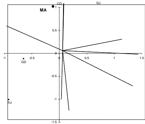
5. Ordination plot for galliformes
