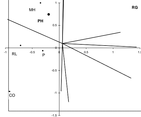
5. Ordination plot for galliformes
