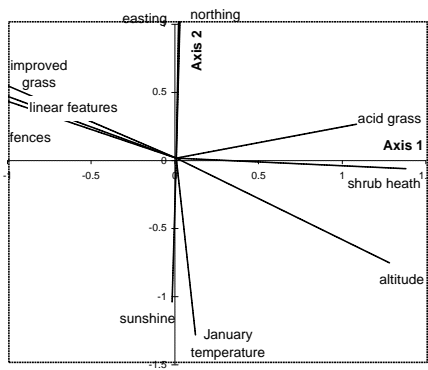
1. Ordination of the ten most significant Environmental Variables
